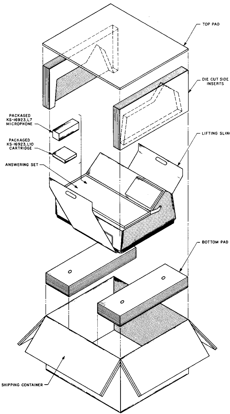
Fig. 1 — Packaging KS-16923, List 1 Telephone Answering Sets
