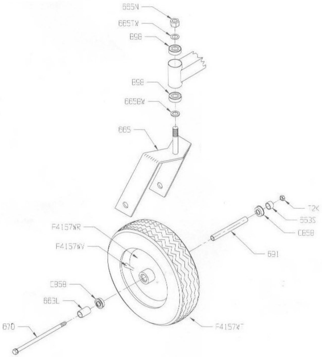
CASTER ASSEMBLY FIGURE 7
