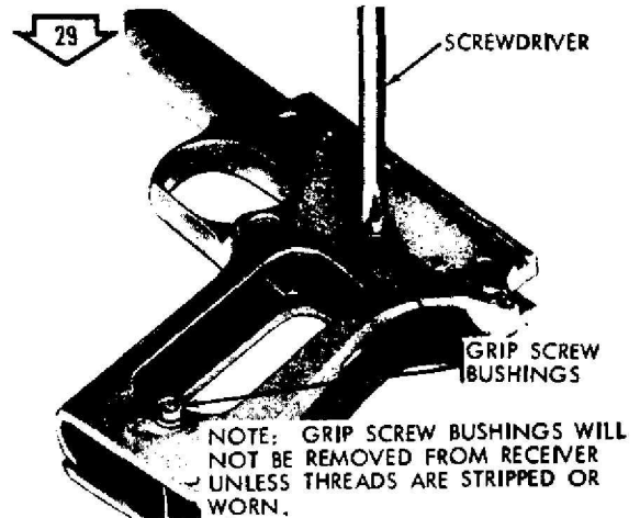
REMOVE GRIP SCREW BUSHINGS.
