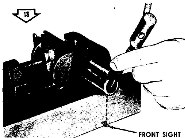
18 • REMOVE FRONT SIGHT.
