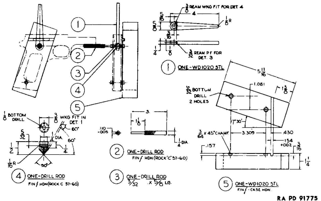
Figure 9. Improvised tool for staking bushing.
