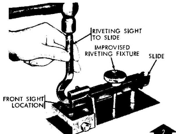
2 INSTALL FRONT SIGHT.
