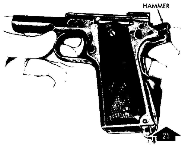
COCK HAMMER PRIOR TO INSTALLING SAFETY.
