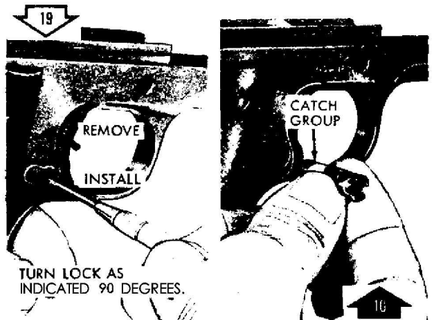
UNLOCK/LOCK CATCH GROUP REMOVE/INSTALL MAGAZINE CATCH GROUP.
