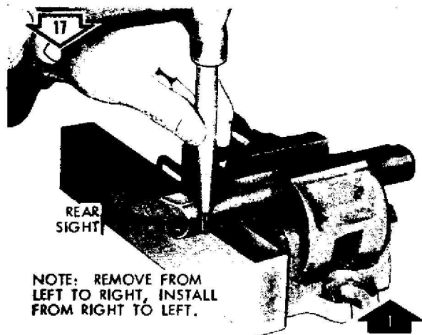
17 REMOVE/INSTALL REAR SIGHT.
