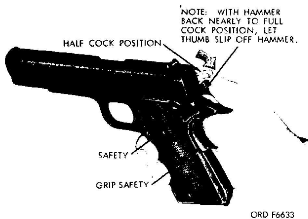
Figure 14. Half-cock position test (2 of 2).
