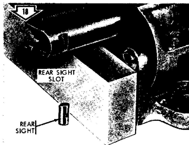
18 REAR SIGHT REMOVED.
