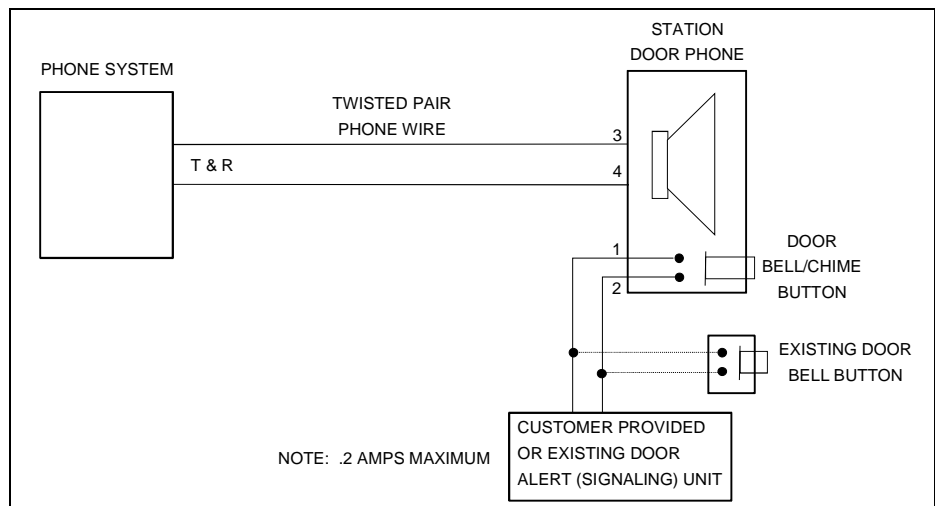
Figure 4. Wiring Diagram for Customer Provided or Existing Alerters
