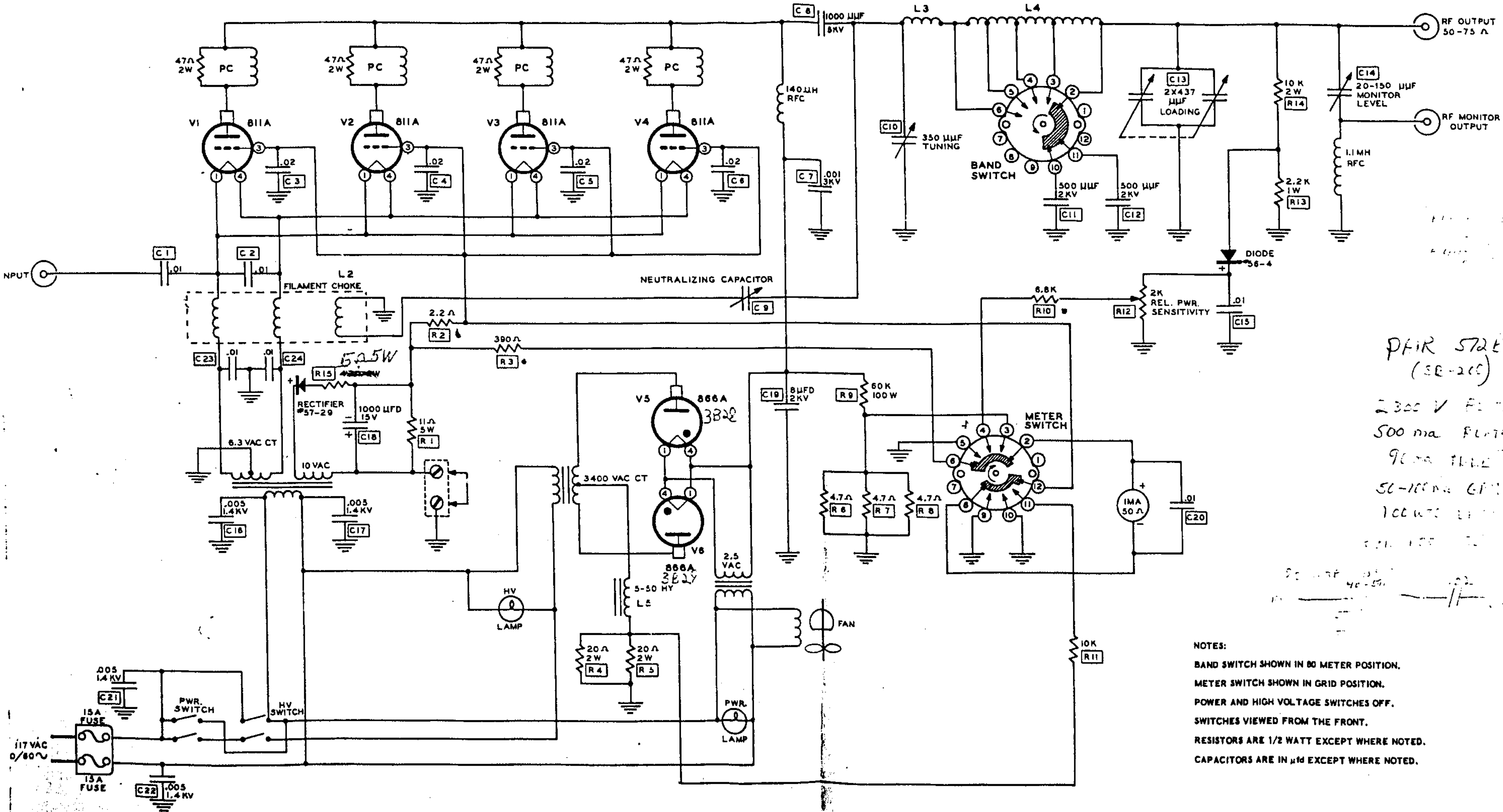
KILOWATT LINEAR AMPLIFIER MODEL HA-10
