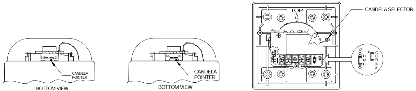
Figure 1: Showing Location of Candela Selector and Jumper Plugs
