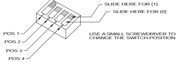
Figure 3: Switch Settings
