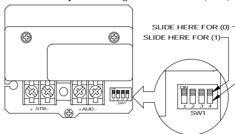
Figure 2: PC Board Layout Showing Location Switch (SW1)
