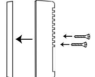
Side view of the E-20A
