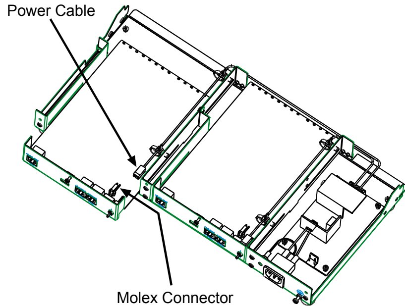
Figure 2: MVP2410/3010 Chassis (top/rear view)
