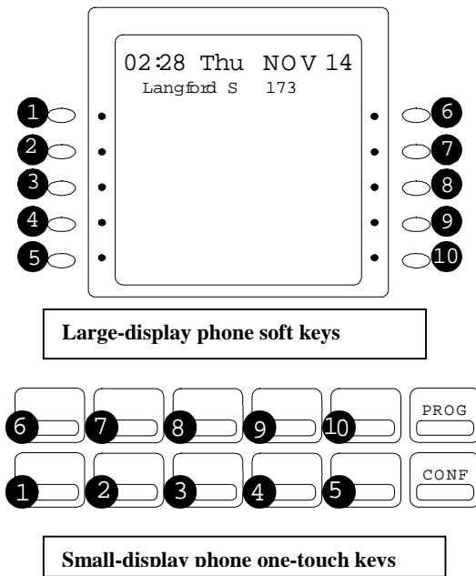
Figure 16. One-touch and soft key numbering scheme
