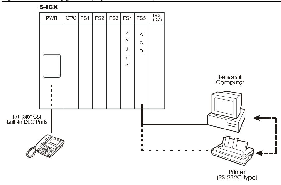
Figure 1. ACD Configuration (96 port cabinet shown)
