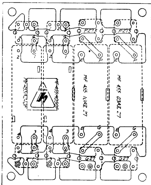
MODE SWITCH
