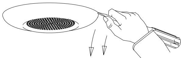
Figure 6: Grille Removal
