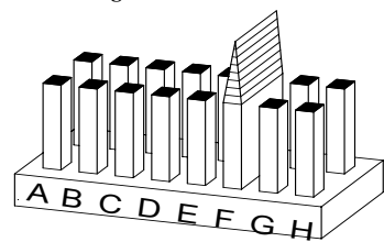
Figure 3: Jumper plug is used to select tap settings which = dBA loudness. Figure 4: Tap Settings (Factory setting is 70V @ 1/2W (Tap F))
